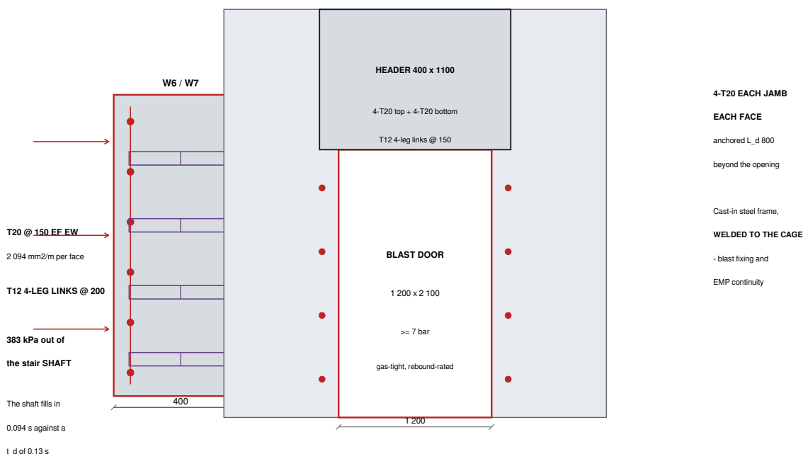
Fig 7.2 : Walls W6 and W7 with the Blast Door Opening
