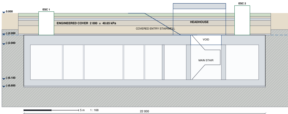
Fig 3.2 : Longitudinal Section on the Box Centreline
