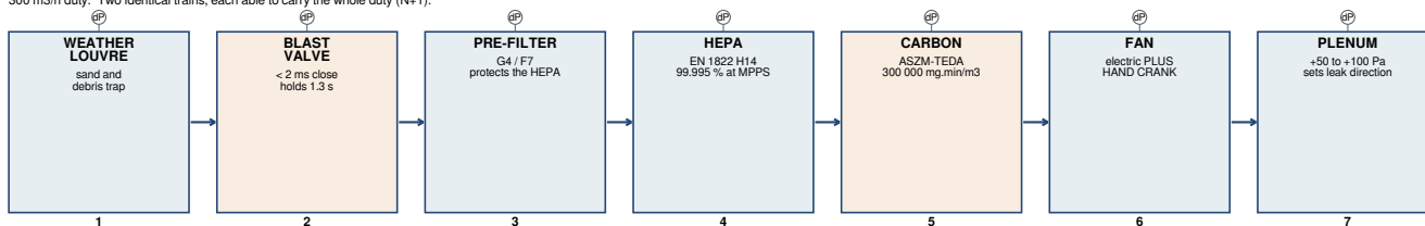
Fig 10.1 : NBC Filter Train, Seven Stages
