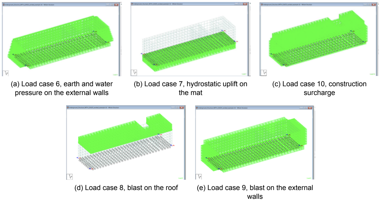
Fig 6.2 : Load Cases 6 to 10, Underground Structure Model (STAAD.Pro)
