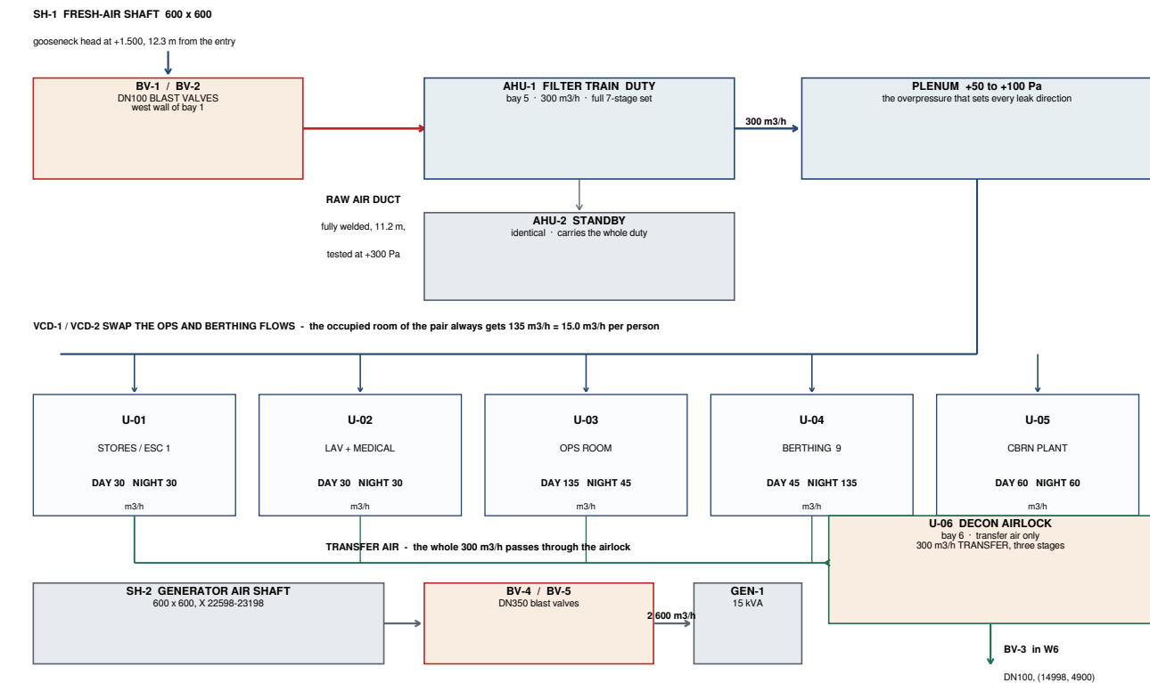
Fig 10.2 : Ventilation Air Path and Room Distribution
