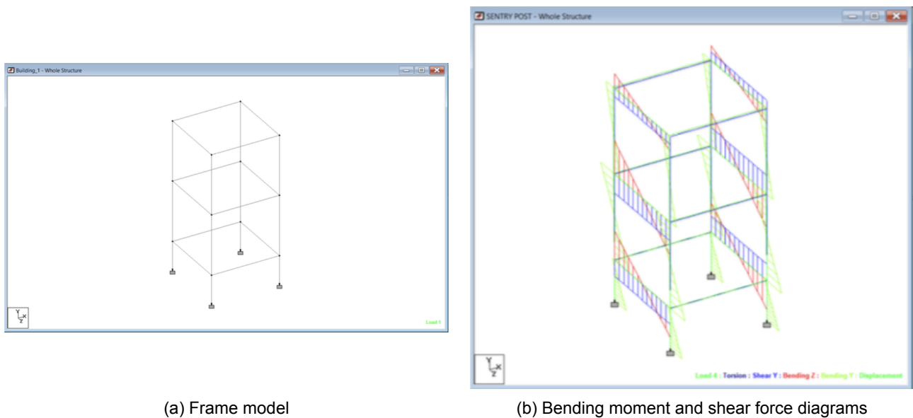
Fig 6.5 : Sentry Post Frame Model (STAAD.Pro)
