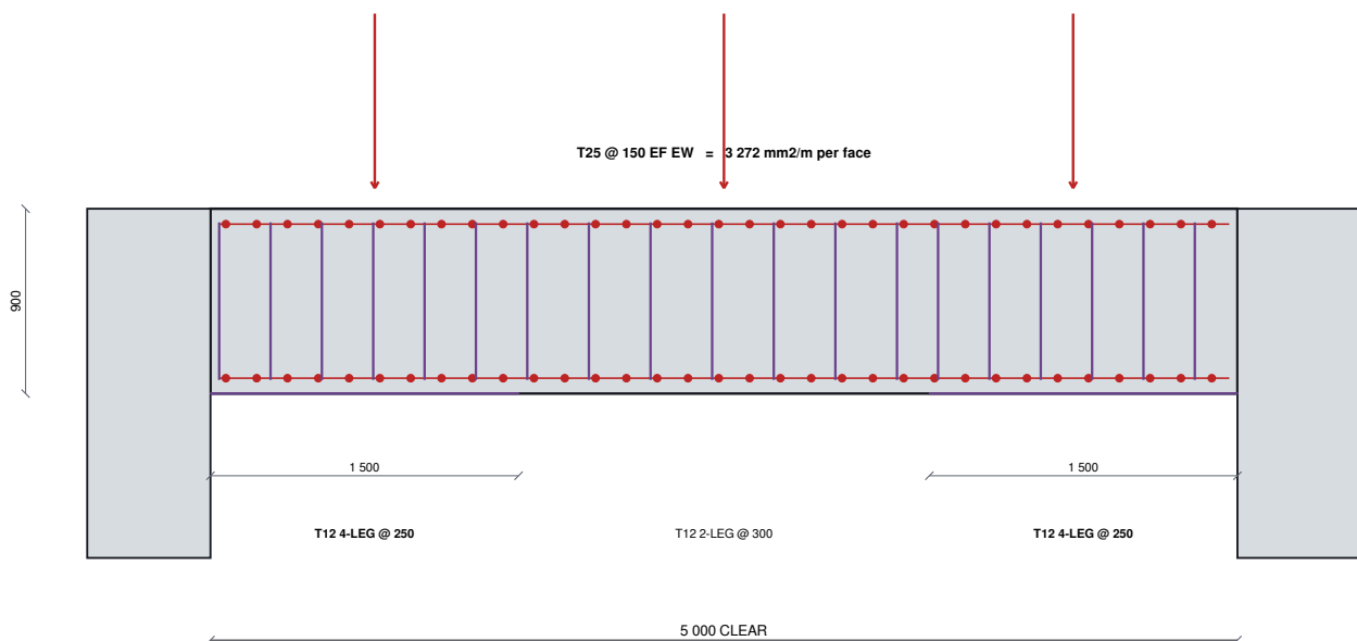
Fig 7.5 : Pressure Slab, Section and Reinforcement
