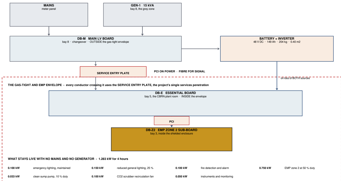
ELECTRICAL SINGLE LINE DIAGRAM - SOURCES, BOARDS AND ESSENTIAL SERVICES
