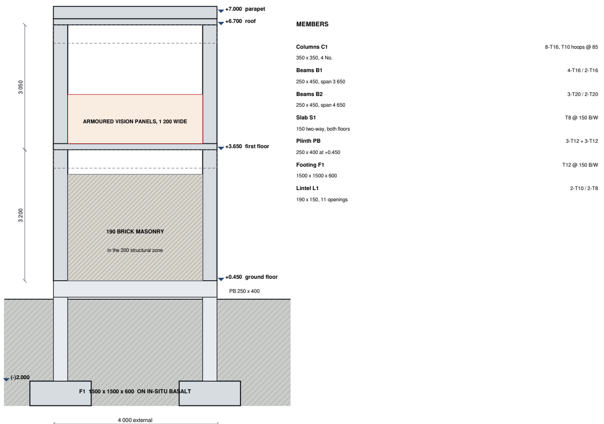
Fig 9.1 : Sentry Post, Two-Storey RC Frame on Isolated Footings
