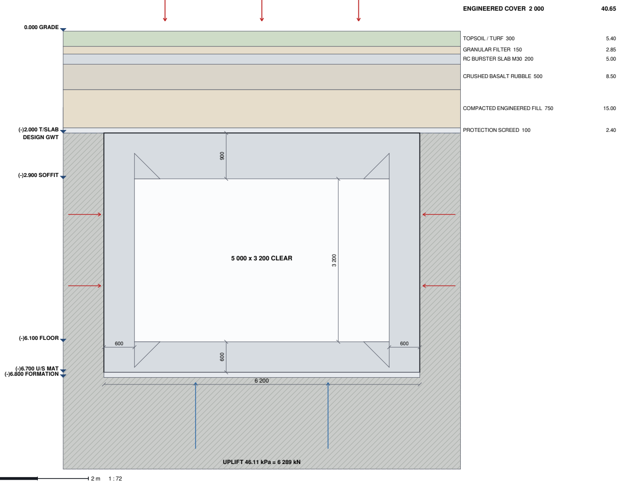
Fig 3.3 : Transverse Section through the Box
