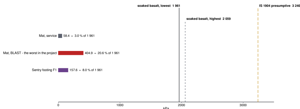
Fig 2.7 : Bearing Demand against Capacity
