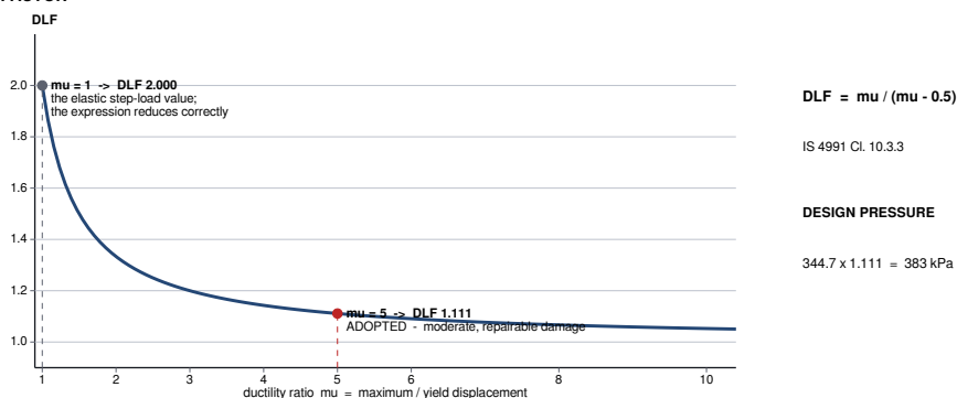
Fig 5.3 : Dynamic Load Factor against Ductility Ratio
