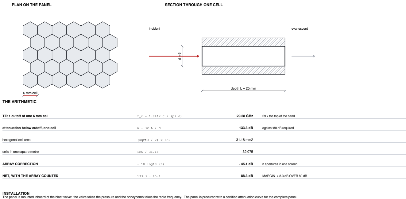
Fig 11.3 : Honeycomb Waveguide Ventilation Panel
