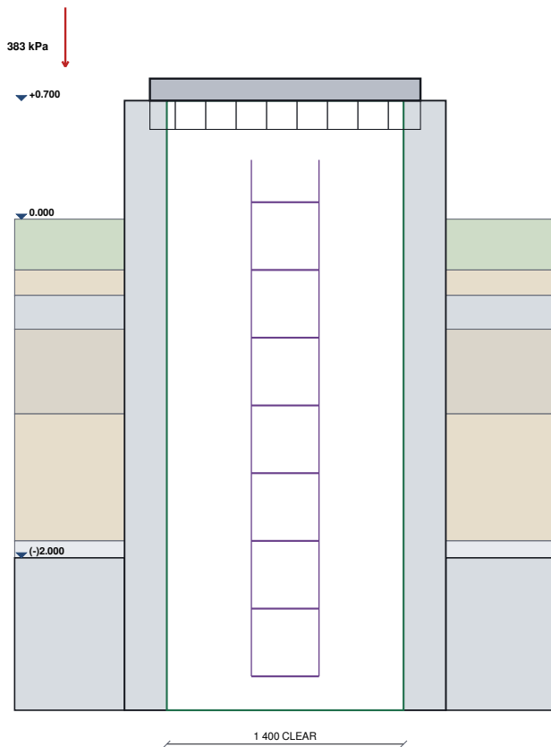
Fig 8.2 : Escape Shaft Head, Hatch and Ladder
