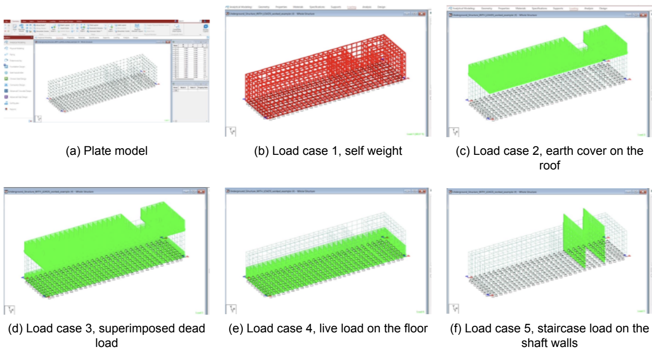
Fig 6.1 : Underground Structure Model and Load Cases 1 to 5 (STAAD.Pro)
