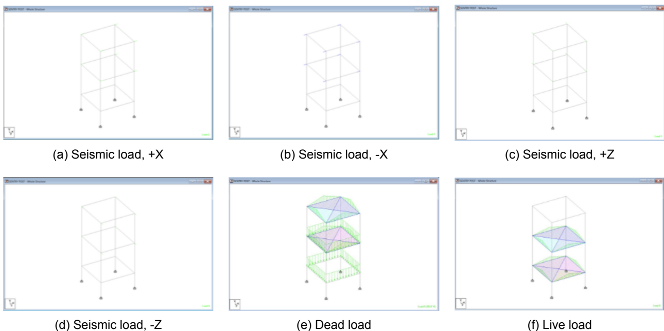
Fig 6.6 : Load Cases, Sentry Post Frame Model (STAAD.Pro)
