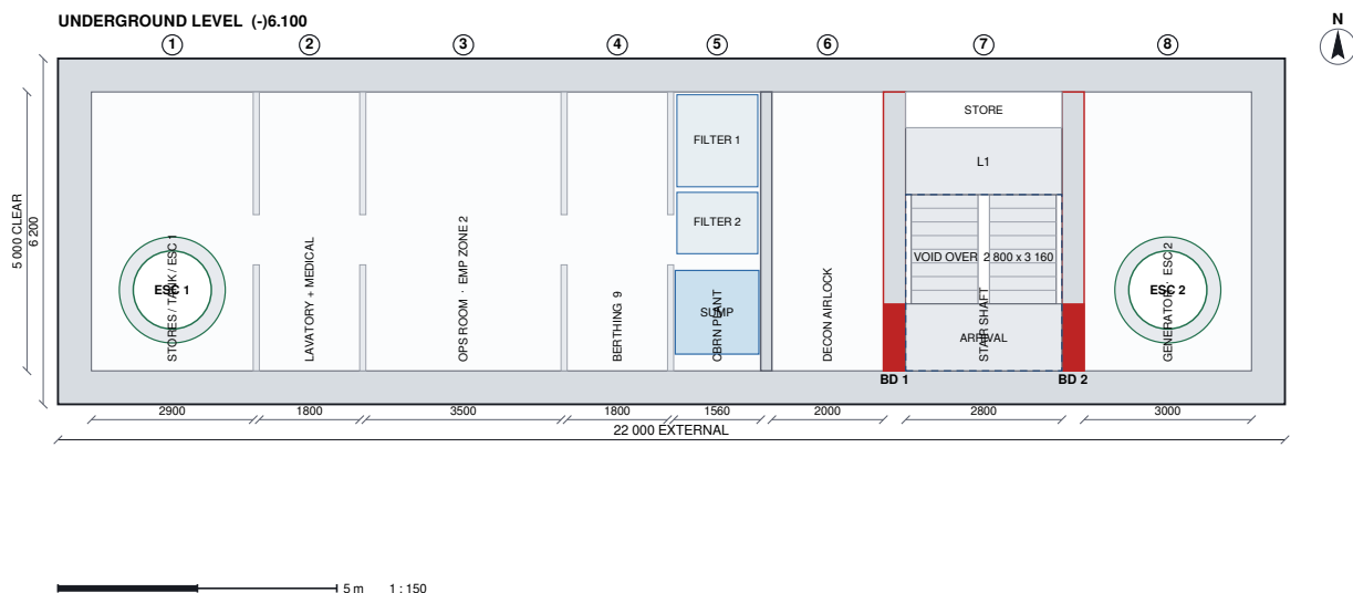
Fig 3.1 : Underground Level Plan at (-)6.100
