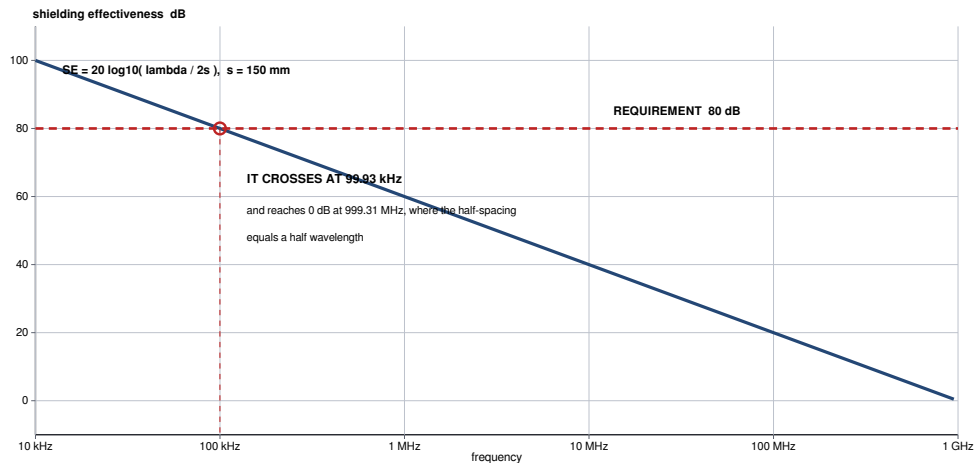
Fig 11.2 : Shielding Effectiveness of the Reinforcement Cage
